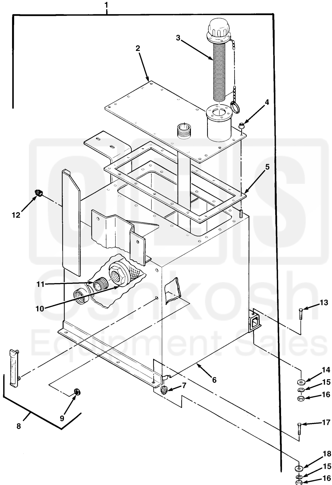
FIG.226 HYDRAULIC RESERVOIR ASSEMBLY
